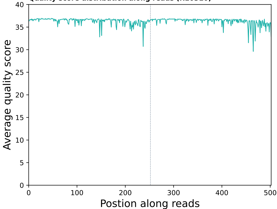
Quality score distribution along reads (R10310)
